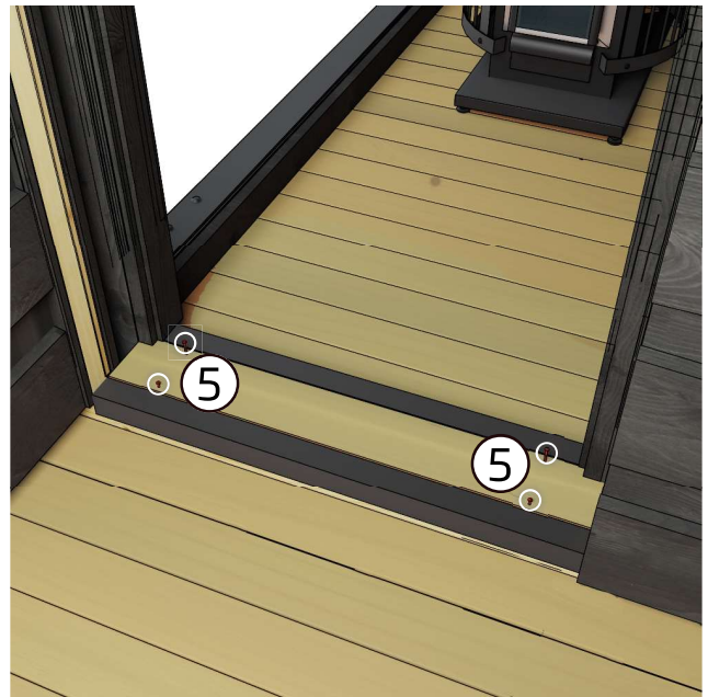
11. Attach the threshold board using screws ( 5 ). The threshold board has pre-drilled holes.
